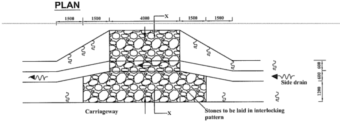
FIGURE C18-ACCESS DRIFT
